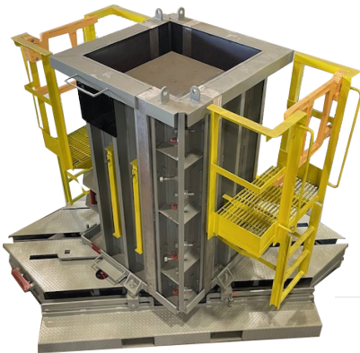
Two Piece Roll Back with Adjustable Wall Thickness
